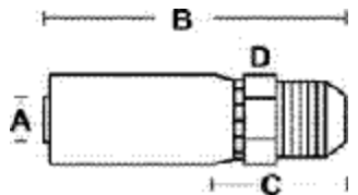
37° JIC MALE RIGID
