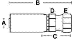
BRITISH STANDARD PIPE 60 CONE FEMALE SWIVEL
