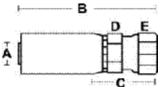
O-RING FACE SEAL FEMALE SWIVEL
