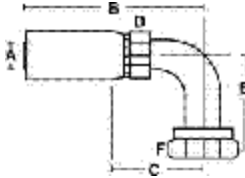
O-RING FACE SEAL FEMALE SWIVEL
