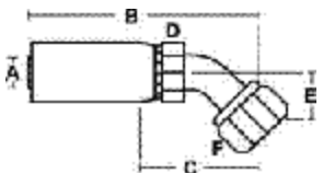
BRITISH STANDARD PIPE 60 CONE 45° TUBE FEMALE SWIVEL
