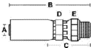
MALE BOSS O-RING SWIVEL
