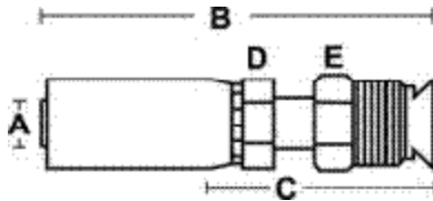
45° SAE MALE INVERTED FLARE 45° BENT TUBE SWIVEL
