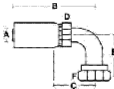
O-RING FACE SEAL 90° FEMALE SWIVEL
