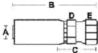
37° JIC FEMALE SWIVEL
