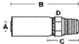
BRITISH PARALLEL PIPE 60 CONE RIGID
