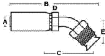
45° SAE MALE INVERTED FLARE 45° BENT TUBE SWIVEL
