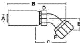
O-RING FACE SEAL 45° FEMALE SWIVEL
