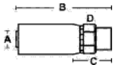
BRITISH FLAT FACE SEAT FEMALE SWIVEL
